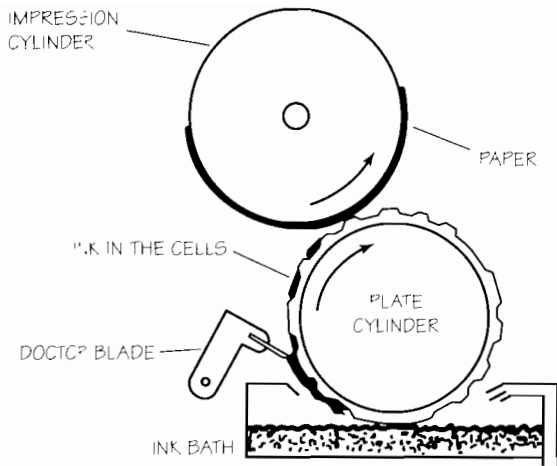
Diagram of a gravure press
